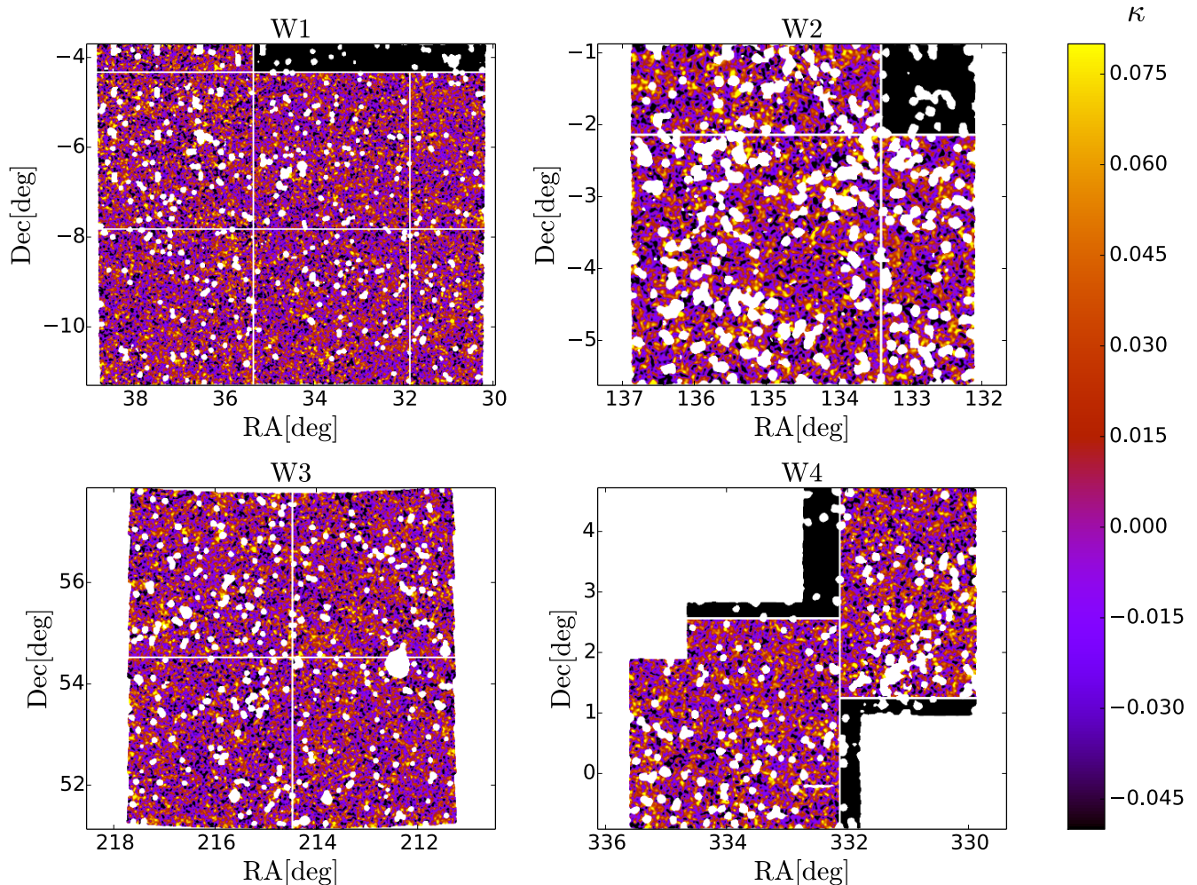
FIG. 1. Convergence maps for the four CFHTLenS fields. They are divided into 13 subfields of 12 deg 2 in size to match our simulation configuration. Scattered white dots are masks. White lines mark the edges of our simulated maps. Three subfields are collages of the six rectangular patches in W1, W2, W4. Patches in black and white are not used in our simulation.
