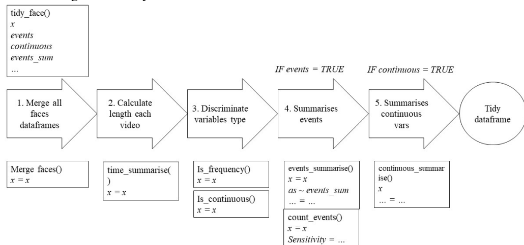
Fig. 3 tidy_face architecture
