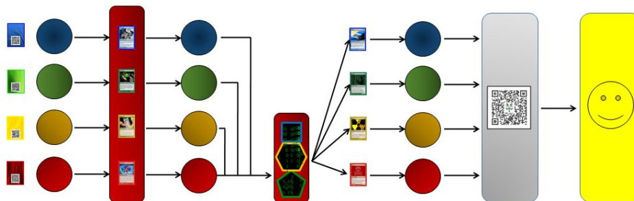
Figure 8. Breakout steps.
