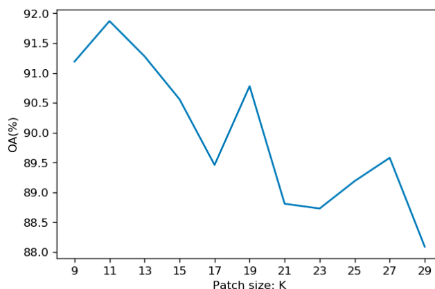
Figure 5. Patch size k vs. overall accuracy.
