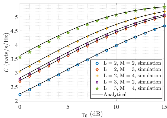
(c) Channel capacity versus \bar{\gamma}_0
