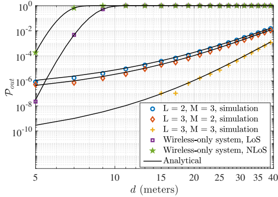
(a) P_{out} versus different propagation distance
