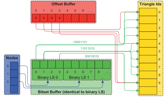
Figure 3: The sparse memory layout of our structure. Nodes have references to their bitsets (shown in green), which signal whether associated shafts are filled or empty. To access the triangle data, an additional offset per bitset is needed (shown in red).
