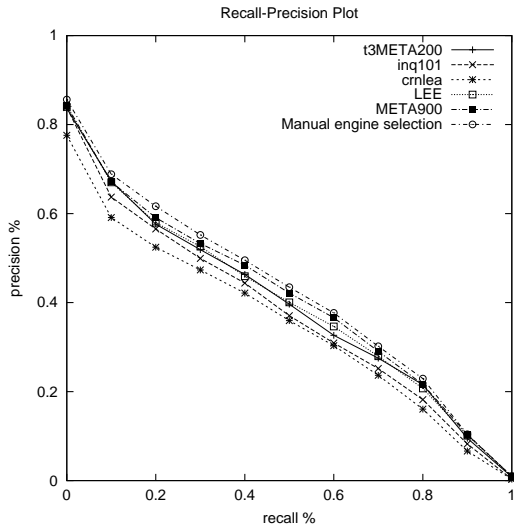
Figure 10: Recall precision graphs for combining inq101 and crnlea using different techniques (see text). Data from TREC-3
