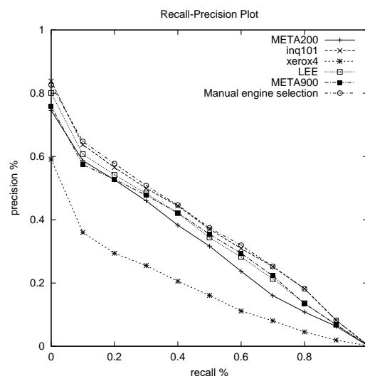
Figure 13: Recall precision graphs for combining inq101 and xerox4 using different techniques. Data from TREC-3.
