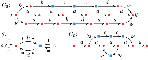
Figure 4: Simple witness for satisfiability.
