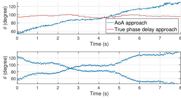
Figure 11: By artificially modifying the signal phase, a transmitter can trick a BLE 5.1 receiver into measuring an arbitrary crafted angle even if not moving (top). A simple approach to detect misleading devices involves changing antenna switching pattern (bottom).
