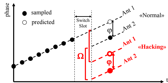
Figure 10: The transmitter can control the phase-delay computed at receiver by modifying phase after switching time, thus compromising correct AoA detection.
