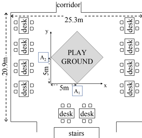
Figure 4: Indoor testbed used for evaluating the AoA-based positioning mechanism. Two receivers (anchors) A_1 and A_2 determine the position of target transmitter in the “playground”.
