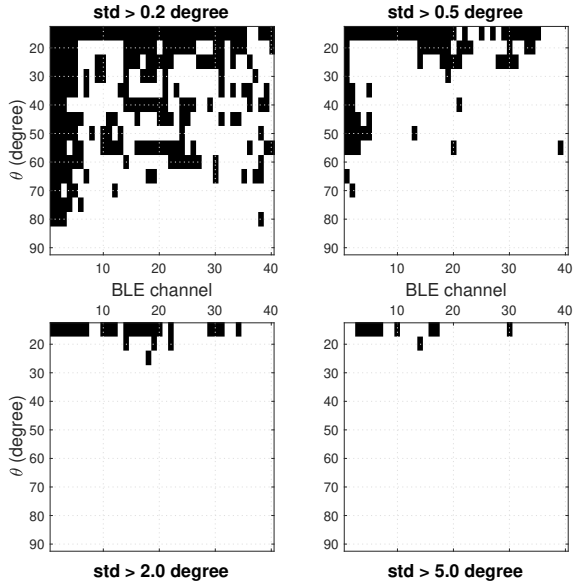
Figure 5: Channel (x-axis) and angle (y-axis) combinations for which the standard deviation of the estimated angle over 30 measurements is below (white) or exceeds (black) the standard deviation threshold indicated in the sub-plot title.
