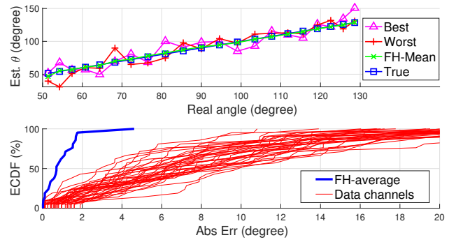
Figure 7: Indoor results for angular accuracy: top, qualitative match of average estimation to True angle; bottom, ECDF of absolute error.
