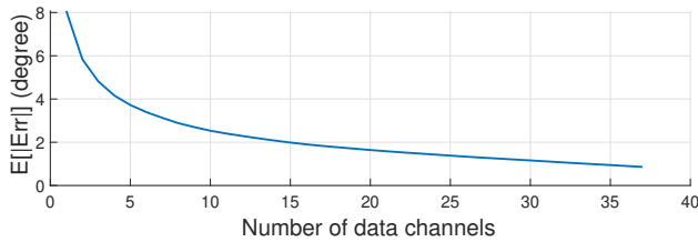
Figure 8: The effect of number of channels used for AoA estimation on the average absolute error.
