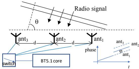
Figure 1: The AoA mechanism needs to estimate phase-delay \varphi between antennas to compute angle \theta : multiple antennas are connected to a single radio transceiver using an RF switch.
