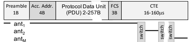
Figure 2: The format of a packet supporting AoA detection, and corresponding switching timing.
