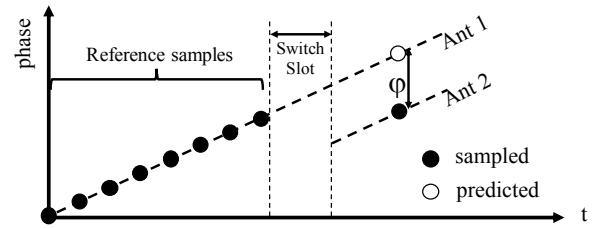
Figure 3: The phase difference is computed by subtracting the phase sampled on antenna 2 from the phase predicted on antenna 1 according to the samples it received during the reference period.
