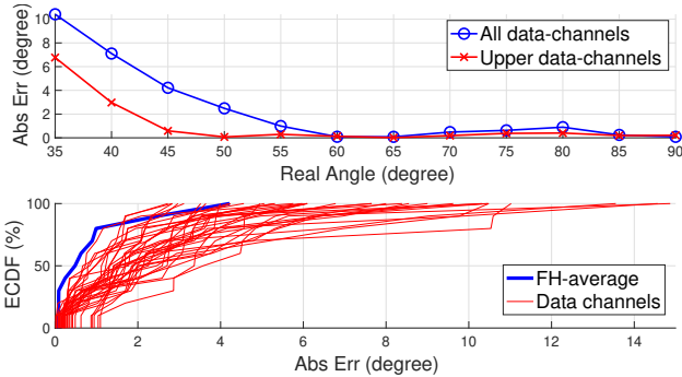
Figure 6: Estimation errors in outdoor settings. Top: absolute error after averaging over all data channels (blue) and over upper-frequency half (red); bottom: ECDF of error after averaging over all data channels and for each channel; angles of 35° and 40° removed.
