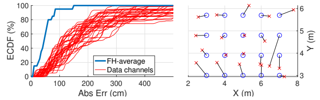
Figure 9: ECDF of indoor position estimation error (left). Qualitative estimation, real (circles) vs estimated (crosses) positions.
