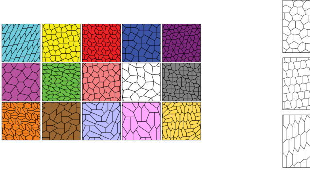
FIG. 3. (Left) The fifteen kinds of tiling pentagons (Source https://commons.wikimedia.org/wiki/File:PolygonTilings15.svg ). (Right) The three kinds of tiling hexagon (Source http://mathworld.wolfram.com/HexagonTiling.html )
