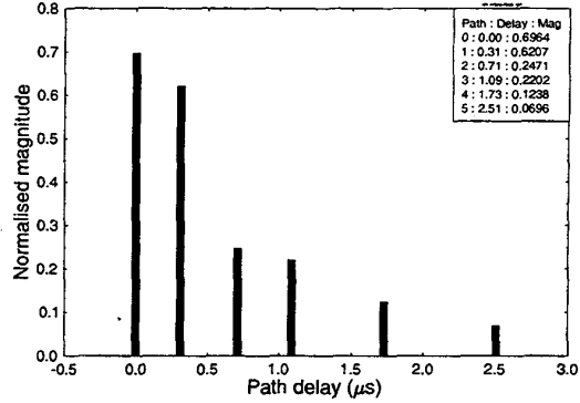
Fig. 1. UTRA vehicular channel A [22].
