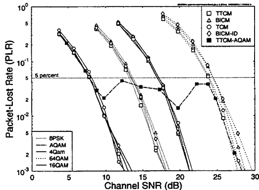
Fig. 3. Packet loss ratio versus channel SNR for the four fixed modulation modes, using the four joint coding/modulation schemes considered, namely BICM-ID, BICM, TCM and TTCM, when communicating over the UTRA channel of Figure 1.
