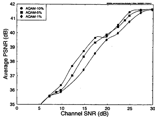
Fig. 6. Average PSNR versus channel SNR for four-mode TCM AQAM scheme in 1%, 5% and 10% packet loss representation.
