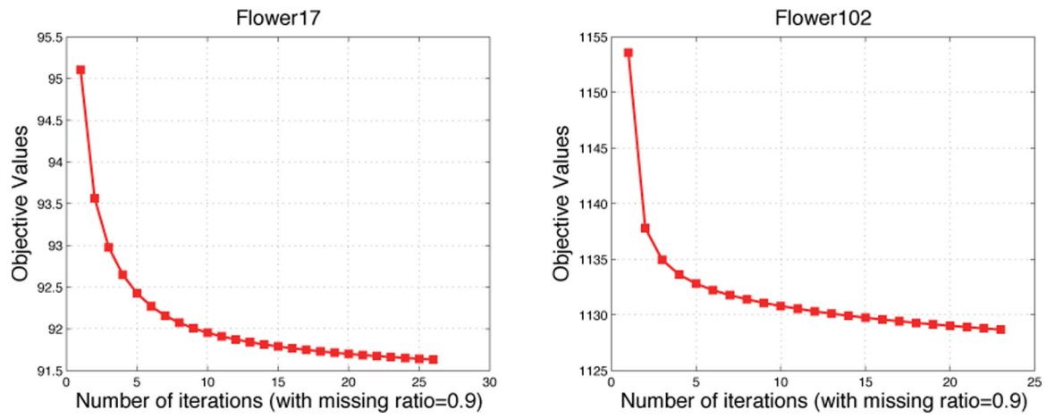
Figure 3: Evolution of the objective value in our algorithm.
