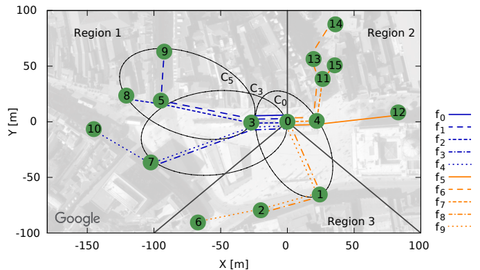
Fig. 9: Lamppost small cell backhaul deployment in Nottingham city centre, operating on mm-wave links. Geographic information extracted from open data set [55]; backhaul carries 10 aggregate flows; cliques of interest circled; topology ‘partitioned’ into 3 regions.
