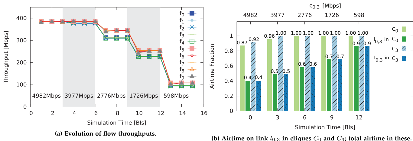
Fig. 11: Flow throughputs and airtime fractions allocated to flow segments traversing l_{0,3} in both cliques, as l_{0,3} degrades. Flow demands remain at 400Mbps. MCS used with different link conditions labelled on white/shaded areas or shown as top x-ticks. Simulation results.
