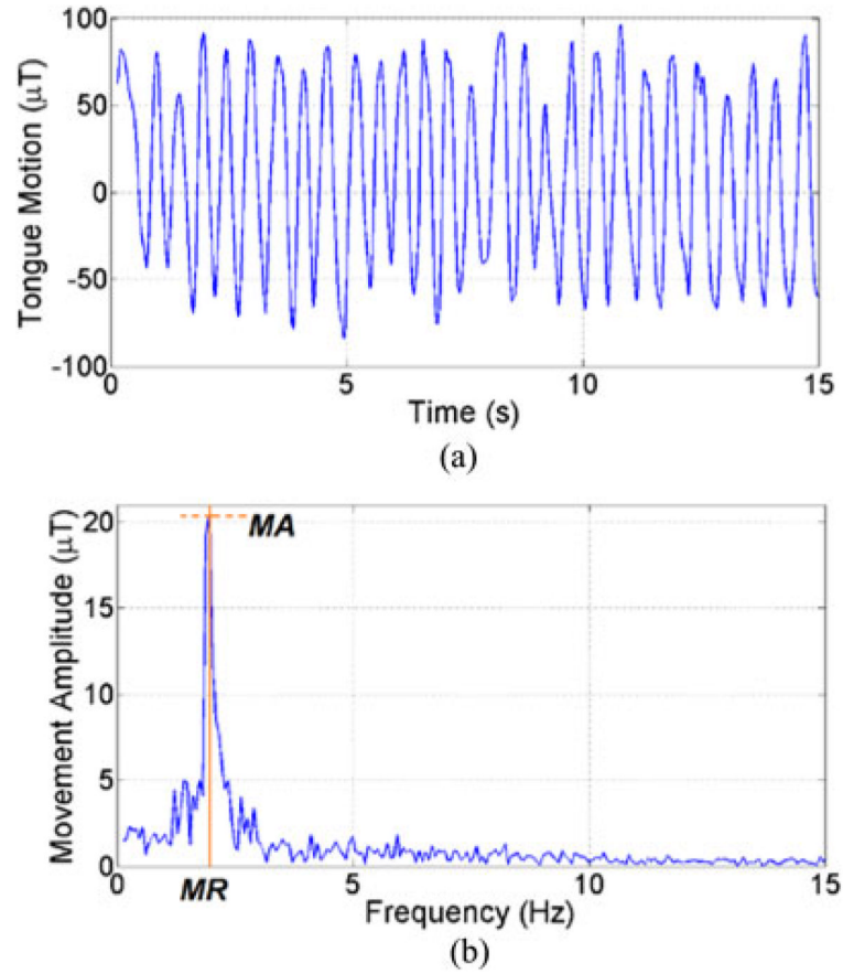
Fig 5. (a) Typical tongue rapid movement waveform and (b) its spectrum derived by FFT. Units are in microtesla because the amplitudes are directly derived from magnetic sensor outputs.
