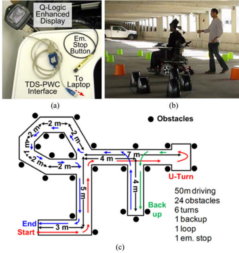
Fig 6. (a) TDS-PWC interface attached to a Pride Q6000 enhanced display [also see Fig. 1(e)]. (b) Experimental setup for the PWC driving part of each session. An operator walked behind the subject with an emergency stop button in hand as a safety measure. (c) Plan of the obstacle course showing its dimensions, obstacle locations, and driving trajectory.
