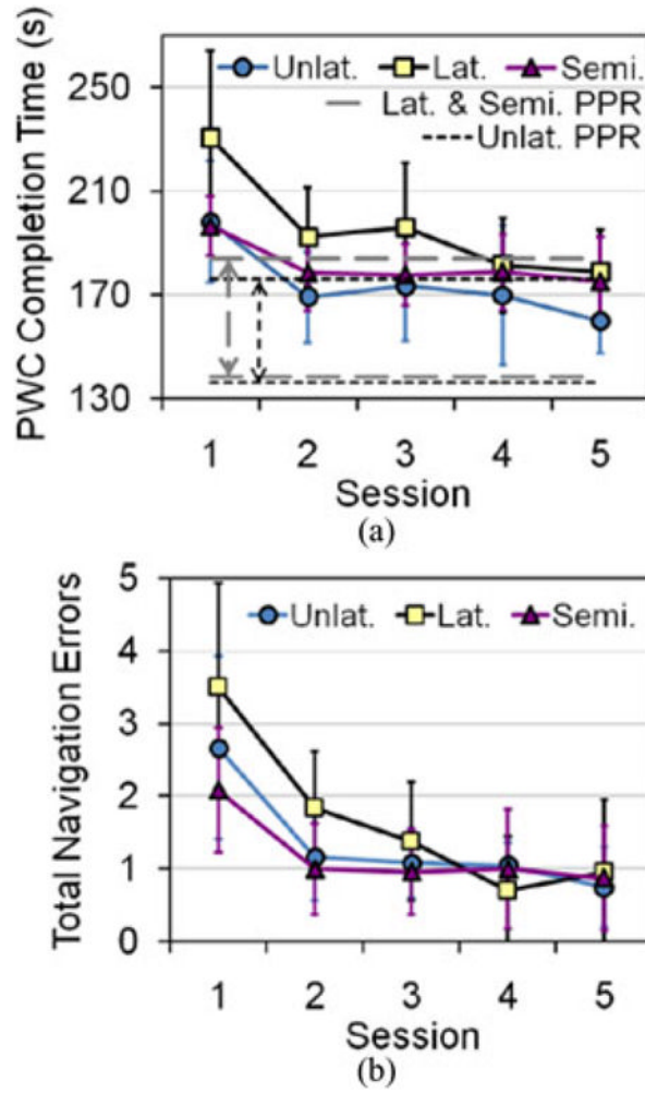
Fig 9. (a) Obstacle course PWC CT and the PPR for various PWC control strategies. (b) Sum of the two types of NEs (collisions and out-of-tracks).
