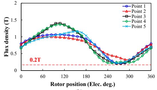
Fig. 11. (a) Field distributions and (b) PM operating points of the proposed ASP-FRPM machine under 2.5 times overload, and temperature=120°C.
