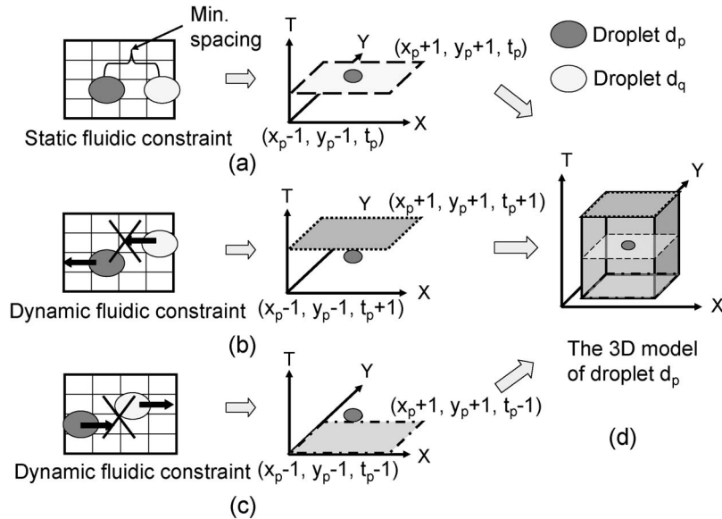
Fig. 4. Example of fluidic constraints. (a) The static fluidic constraint. (b) The dynamic fluidic constraint when a droplet d_q moves to one of the neighboring cells of cell (x_p, y_p) at time t_p . (c) The dynamic fluidic constraint when a droplet d_p moves to cell (x_p, y_p) at time t_p . (d) The 3-D modeling of d_p , where d_p is located at the center of this 3-D cube.
