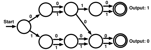
Fig. 1: Sample conjunction program that accepts [0\star 1\star] .
