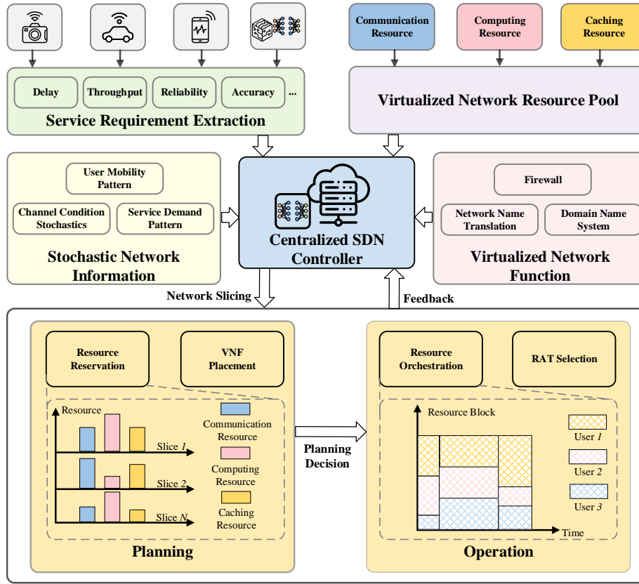
Fig. 2. An illustrative example for the network slicing lifecycle which includes preparation, planning, and operation phases.
