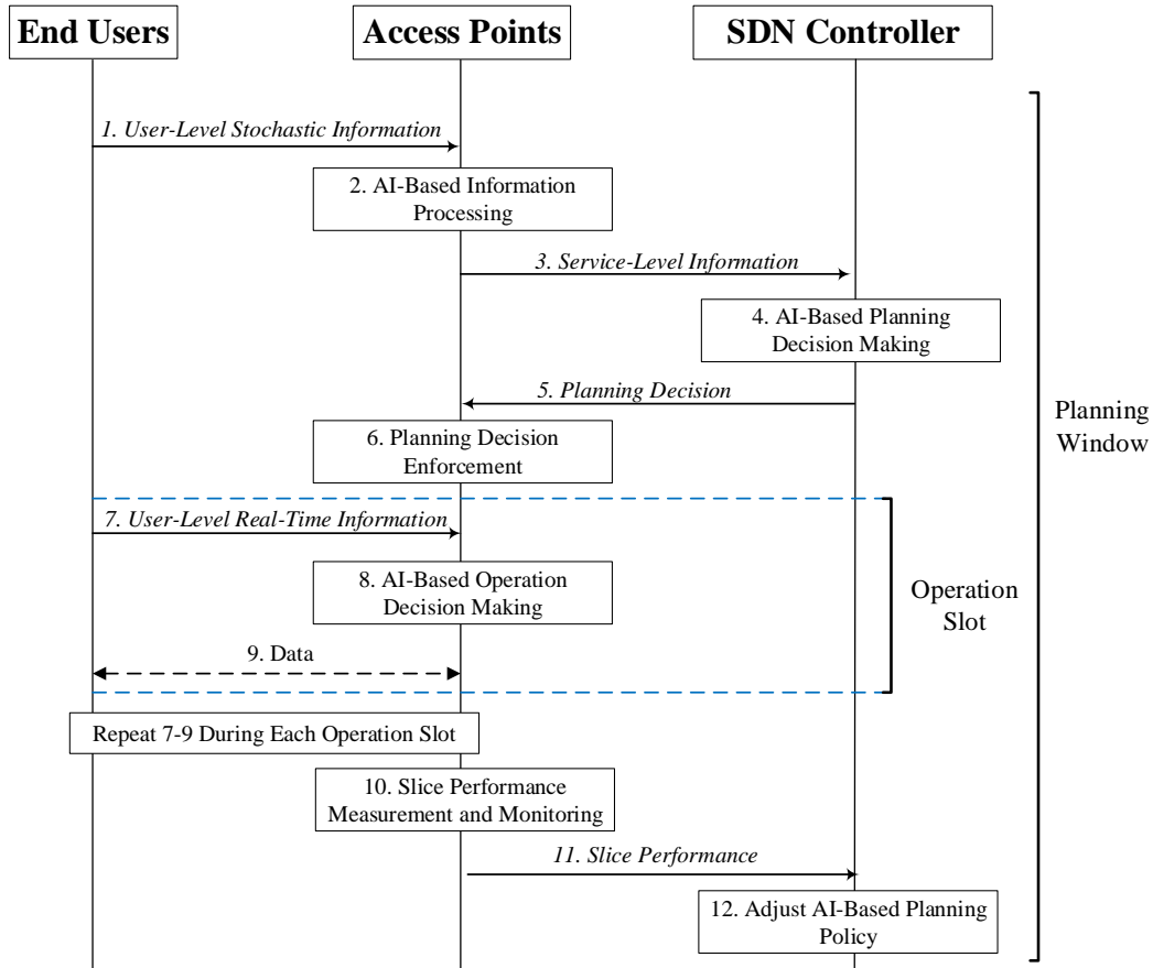
Fig. 4. Procedure of information exchange in AI for slicing.
