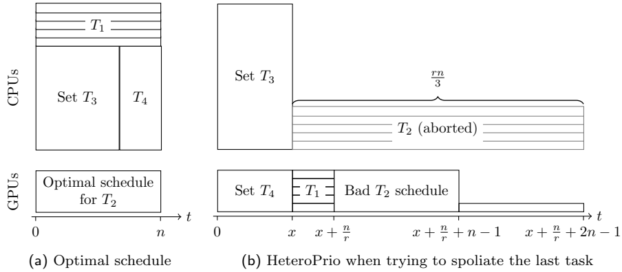
Fig. 5: Optimal and HeteroPrio on Theorem 14 instance
