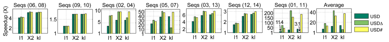
Figure 5. Speedup of our methods against sliding window (SW) in the CMU-Mocap dataset. All 7 pairs of sequences from subject 86 were evaluated. The speedup was computed as the relative number of evaluations N^{SW}/N^{USD} using \ell_1 , \chi^2 and symmetrized KL divergence.
