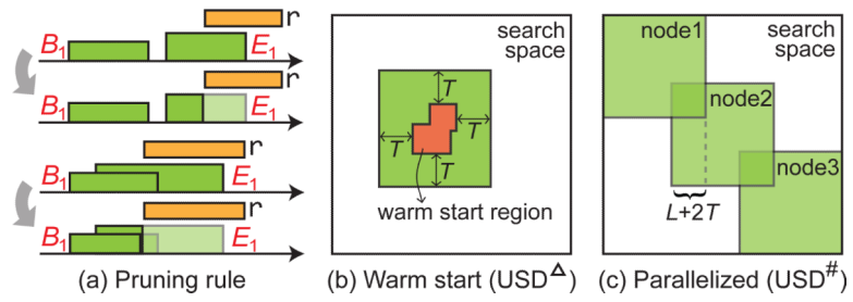
Figure 3. Illustration of USD extensions: (a) pruning rules applied to multi-synchrony discovery, (b) USD with warm start (USD Δ ), and (c) parallelized USD (USD # ).
