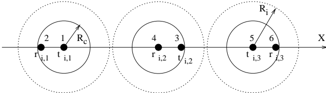
Fig. 1. Graph-Based algorithms can lead to high cumulative interference.
