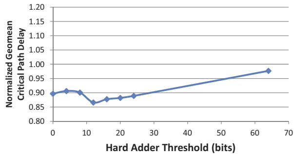
Fig. 5. Circuit speed vs. hard adder threshold. Results are the average across 14 benchmarks and normalized to the soft implementation.
