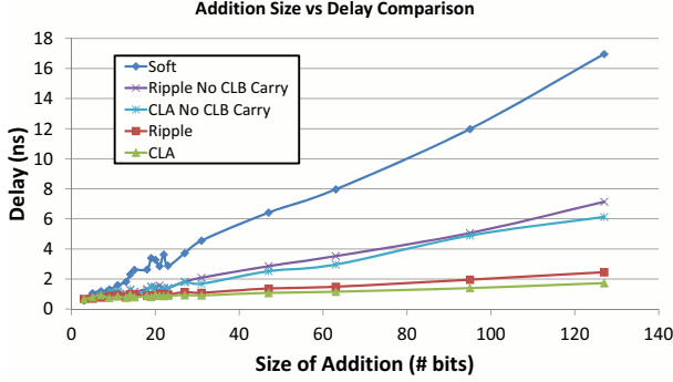
Fig. 8. Delay vs adder length for various architectures.
