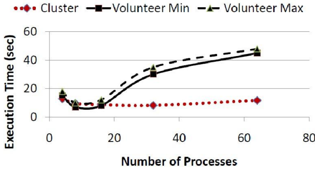
(a) Scalability
