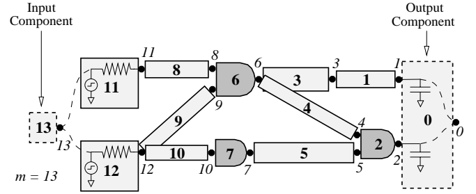
Figure 2: The circuit in Figure 1 with factitious components, node indexes and component indexes.
