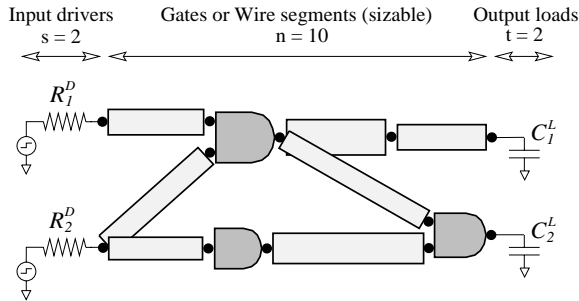
Figure 1: A combinational circuit.
