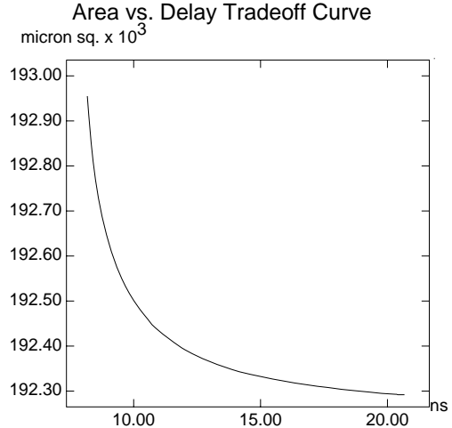
Figure 9: The area vs. delay tradeoff curve for a 16-bit adder.
