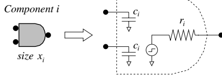
Figure 3: The model of component i , which is a gate, by a switch-level RC circuit. Although the gate shown here is a 2-input AND gate, the model can be easily generalized for any gate with any number of input pins.
