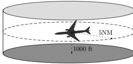
Figure 4 Separation norm for en-route traffic. No other aircraft must enter this volume.
