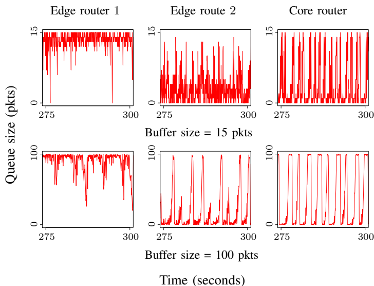
Fig. 21: Queue size dynamics with long-lived flows : Two sets of 60 Compound TCP flows each with an access speed of 2 Mbps, regulated by two edge routers each with a link capacity of 100 Mbps, and feeding into a core router with a link capacity of 197 Mbps. The flows in the two sets have average round trip times 10 ms and 200 ms respectively. It can be easily noted that as buffer sizes are increased from 15 to 100 packets, the queue size dynamics exhibits limit cycles.
