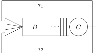
Fig. 8: Single bottleneck topology with heterogeneous round trip times. Two sets of TCP flows with round trip times \tau_1 and \tau_2 , feeding into a common bottleneck router. The buffer size at the router is B and the link capacity is C .
