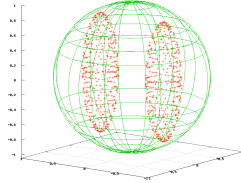
Figure 2: A pair of triangulated ellipsoids define a bounded domain D_1 that lies within an enclosing sphere S_1 . The scattering matrix for D_1 will be created on S_1 and used to represent the exterior field.
