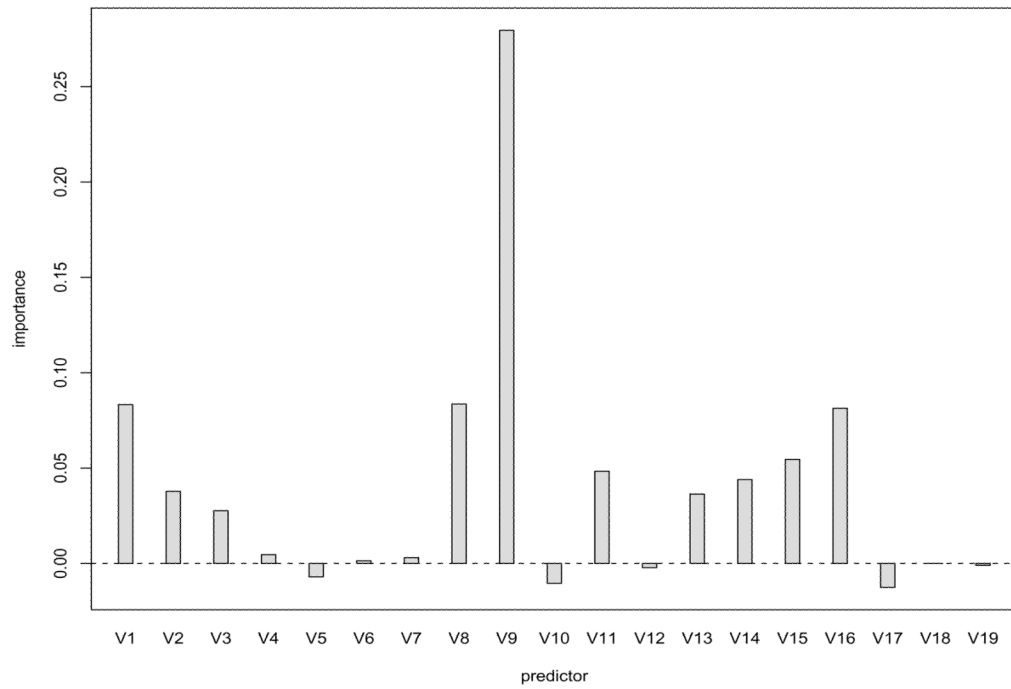
Figure 4. Variable importance measures in the DLS data obtained via random forests.
