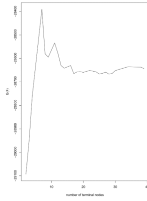
Figure 2. Tree size selection for the DLS data: Plot of G(4) versus the tree size
