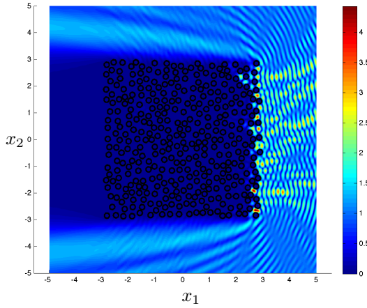
(c) Sound-soft problem: |u^{\text{tot}}|
