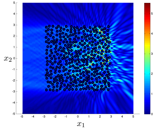
(f) Sound-hard problem: |u|
