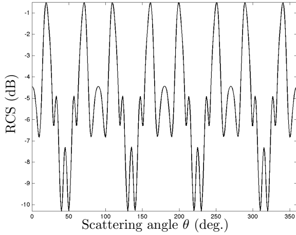
(a) RCS for the penetrable case
