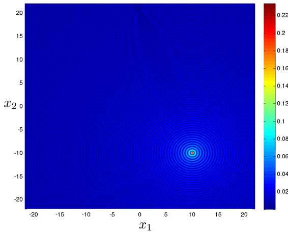
(c) Amplitude of the second Herglotz wavefunction
