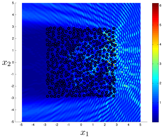
(e) Sound-hard problem: |u^{\text{tot}}|
