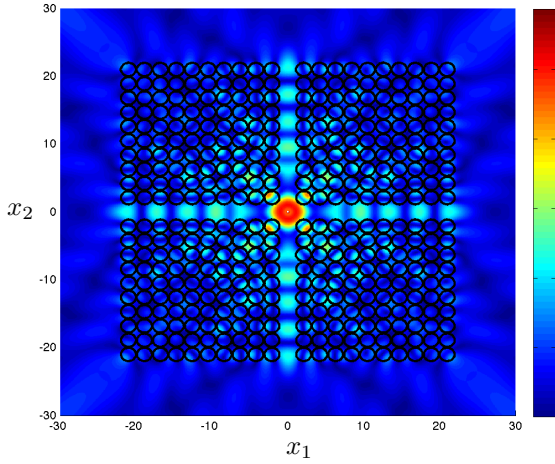
(c) Penetrable problem: \Re(u^{\text{tot}})
