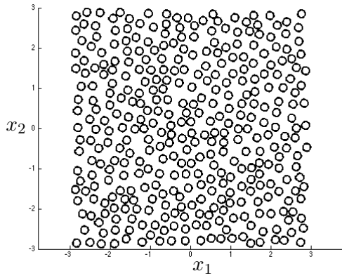
(a) Cluster of M = 360 disks
