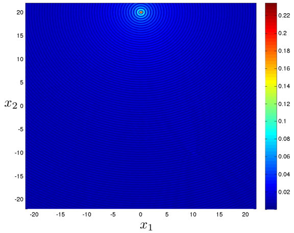
(b) Amplitude of the first Herglotz wavefunction
