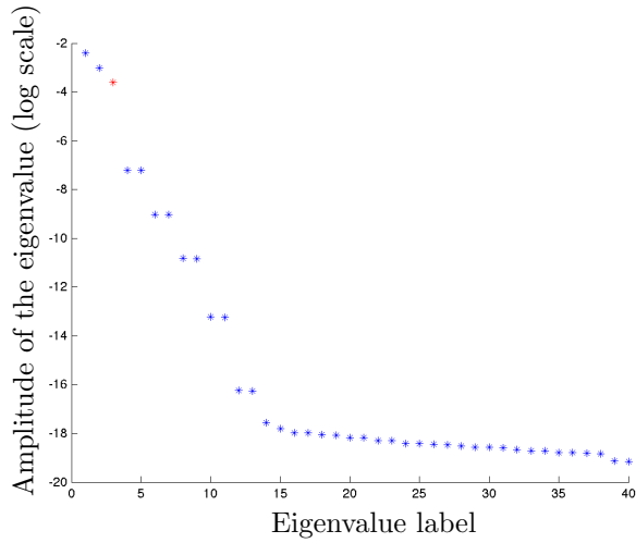
(a) 40 largest eigenvalues of T (log scale)
