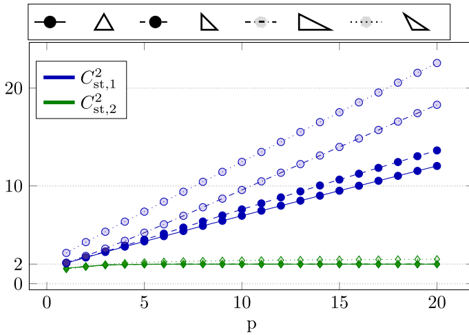
Fig. 1 Approximations of C_{st,1}^2 and C_{st,2}^2 as a function of the polynomial degree p on the equilateral triangle \Delta , the right-isosceles triangle \triangle , \triangleleft, \triangleleft := \text{conv}\{(0, 0), (1.5, 0), (0, 1)\} , and \triangleleft := \{(0, 0), (1, 0), (-1/2, 1)\}
